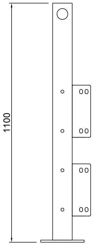
Double Barrier/Handrail
